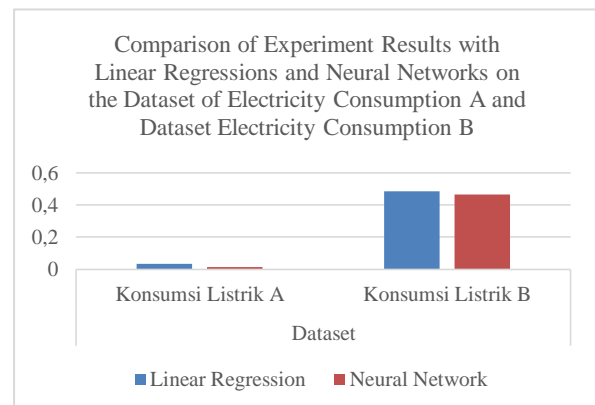
Figure 2 Comparative Graph of Experiment Results of Linear Regressions and Neural Networks on the Dataset of Electricity Consumption A and Dataset Electricity Consumption B
