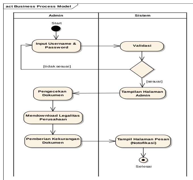
Gambar 5. Activity Diagram Admin Pengecekan Dokumen
