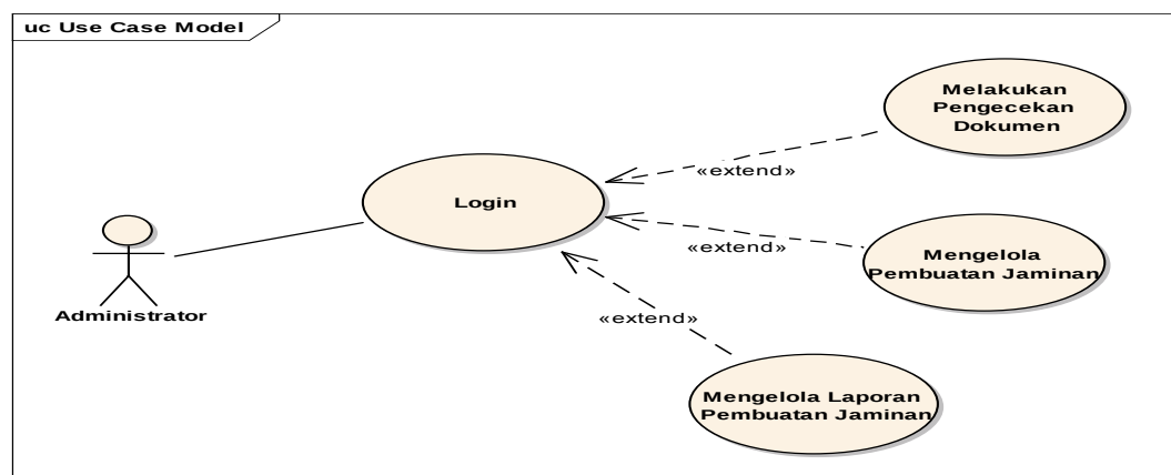
Gambar 3. Use caseDiagram Registrasi Administrator
