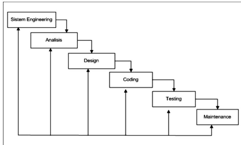
Gambar 1. Waterfall Model
