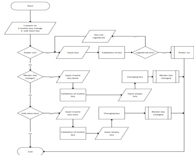
Figure 2. System flowchart Motorized Vehicle Security System
