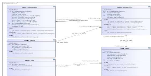
Figure 2. Brainmatics Attendance Data Model
