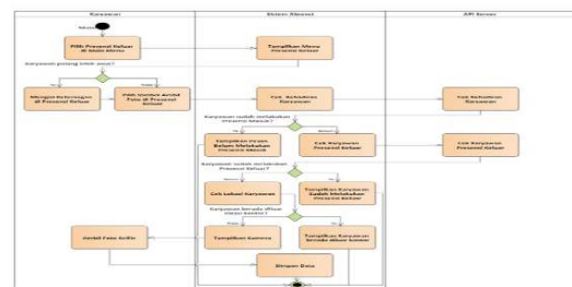
Figure 4. Attendance-Out Activity Diagram
