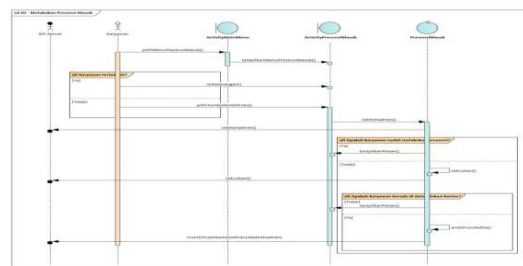
Figure 5. Sequence Diagram perform Attendance-In
