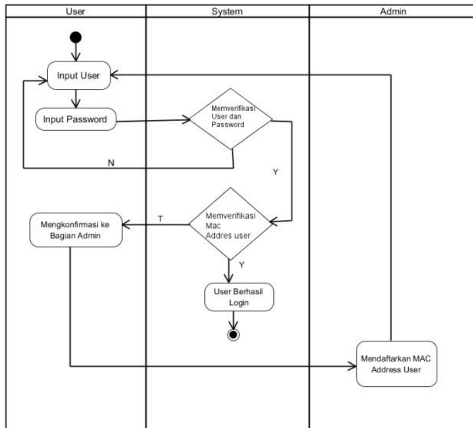
Gambar 1. Activity Diagram
