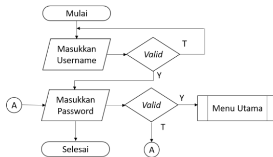
Gambar 10 Flowchart Log In
