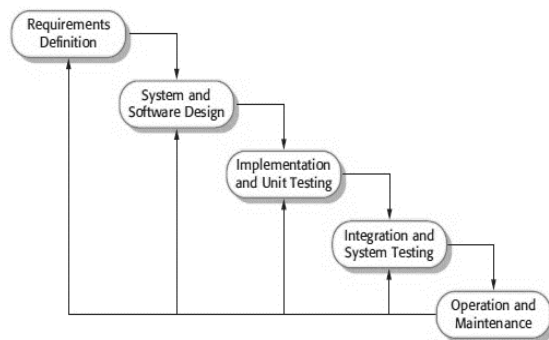
Gambar 1. Model Waterfall
