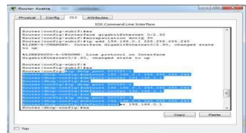
GambarIII. IP DHCP Router Perusahaan
