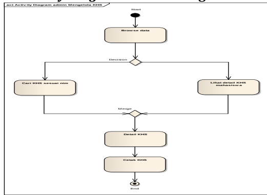
Gambar 11. Activity Diagram Admin Mengelola Data KHS
