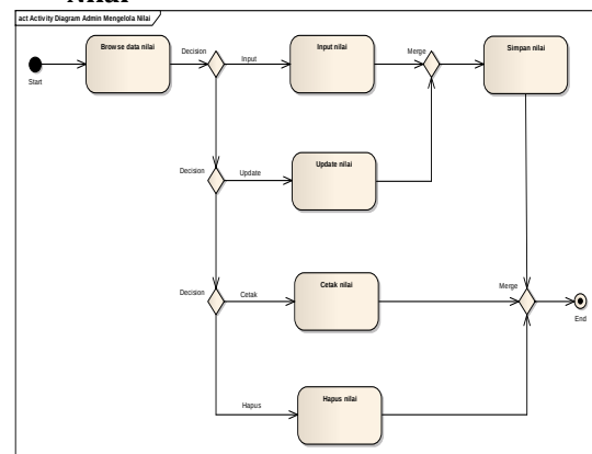
Sumber: (Sastra et al., 2019) Gambar 10. Activity Diagram Admin Mengelola Data Nilai
