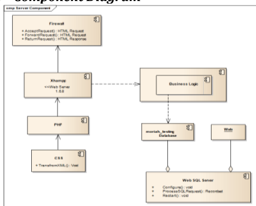
Gambar 13. Component Diagram
