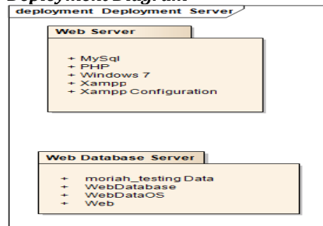
Gambar 14. Deployment Diagram
