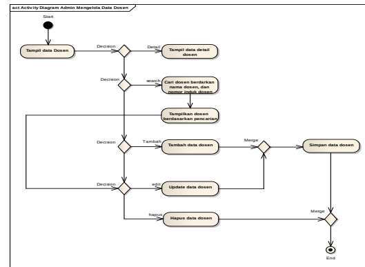
Sumber: (Sastra et al., 2019) Gambar 9. Activity Diagram Admin Mengelola Data Dosen
