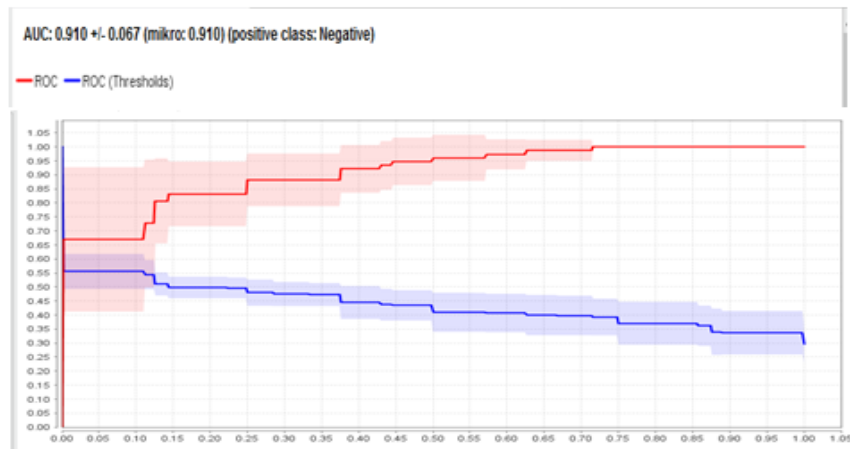
Gambar 9. Kurva ROC Support Vector Machine dan PSO.
