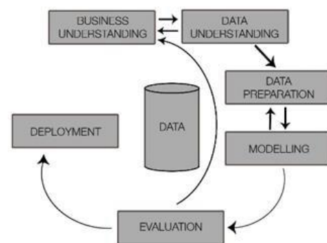
Figure 1. CRISP-DM [27]
