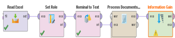
Gambar 8. Menghubungkan fitur selection Information Gain
