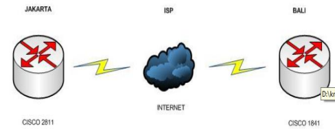
Gambar 1. Topologi routing static
