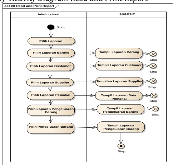
Gambar 9. Activity Diagram Read and Print Report
