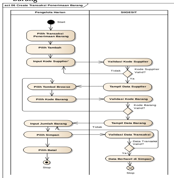
Gambar 7. Activity Diagram Create Transaksi Penerimaan Barang
