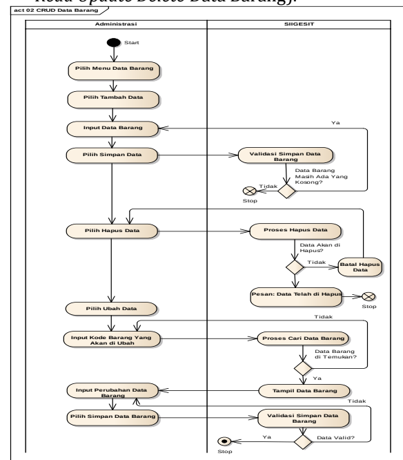
Gambar 3. Activity Diagram CRUD Data Barang
