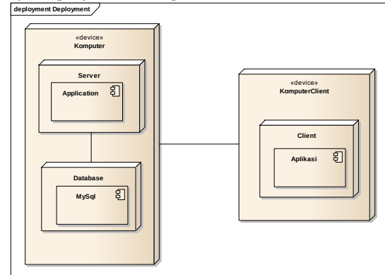
Gambar 13. Deployment Diagram SIIGESIT
