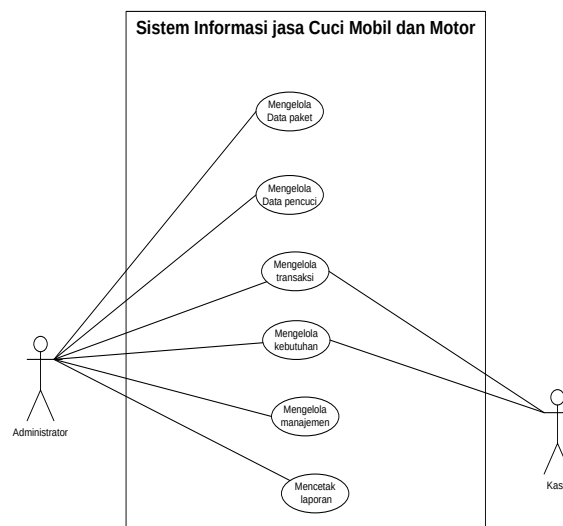
Gambar 2. Usecase diagram
