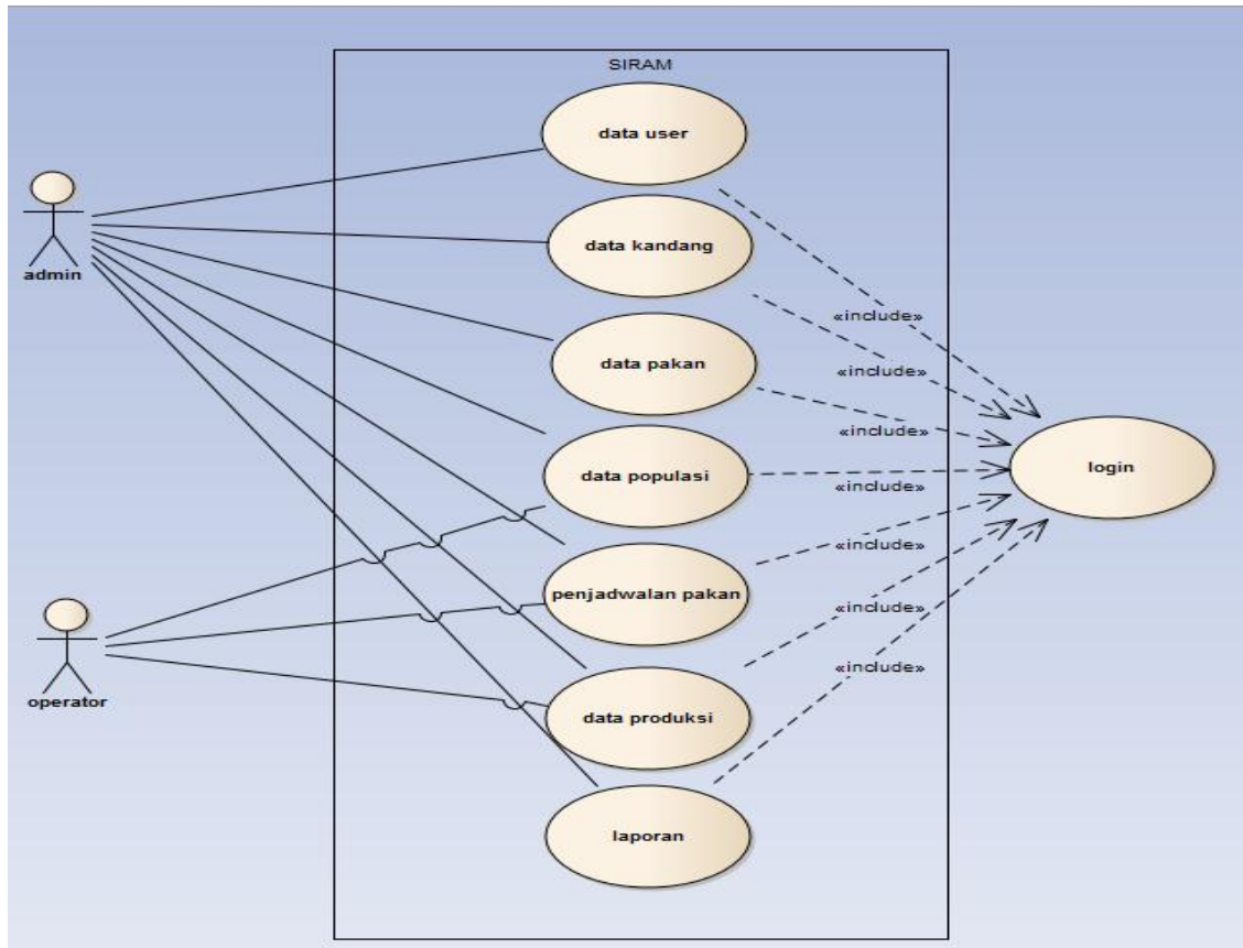
Gambar 5. Usecase Diagram
