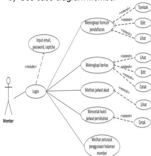
Gambar 2. Use case diagram member
