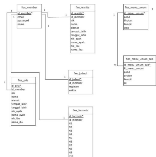
Gambar 11. Logical Record Structure
