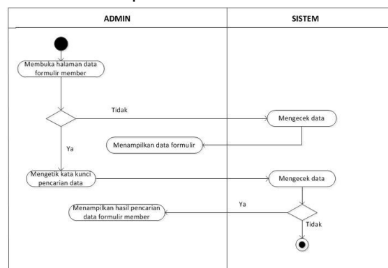
Gambar4. Activity Diagram Admin mengecek formulir pendaftar nikah
