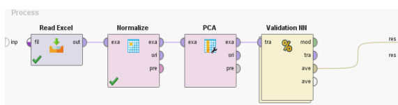
Figure 8. Process Model Method of NN + PCA.
