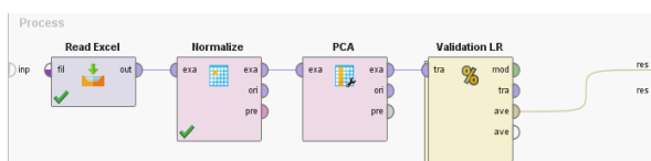
Figure 7. Process Model Logistic Regression + PCA Method.
