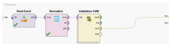
Figure 5. Process Model Support Vector Method.
