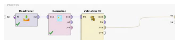
Figure 4. Process Model Neural Network Method.
