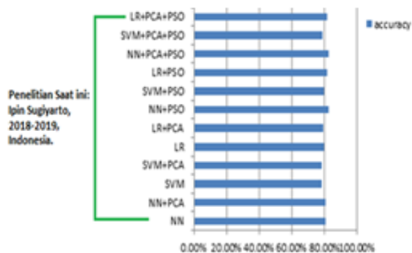
Figure 16. Comparison of Research Accuracy Charts on Approval Credit Cards.
