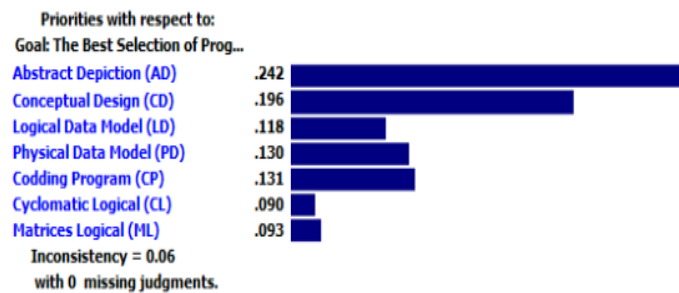
Figure 1. Eigenvector using expert choice
