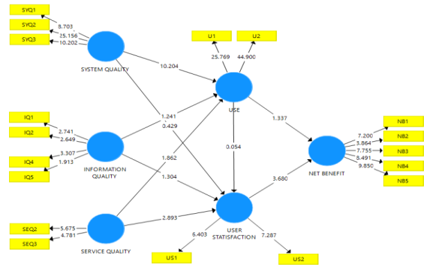
Figure 5. Bootstrapping
