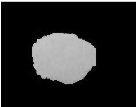
Gambar 7. Citra Biner
