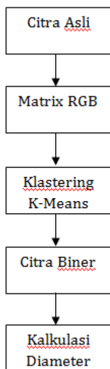
Gambar 1. Metode Penelitian
