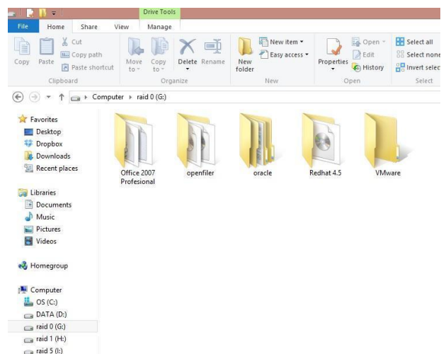
Gambar 9. Isi RAID 0
