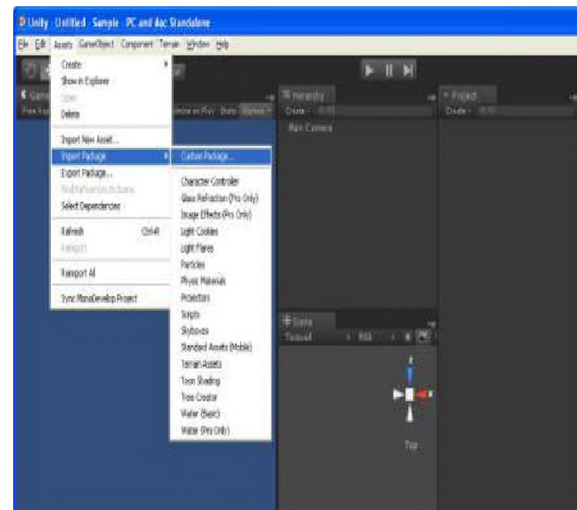
Gambar 15. Import Package
