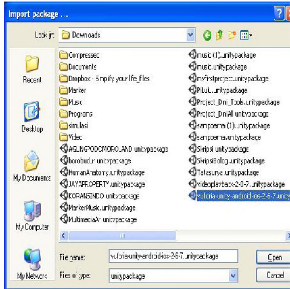
Gambar 16. Import Package
