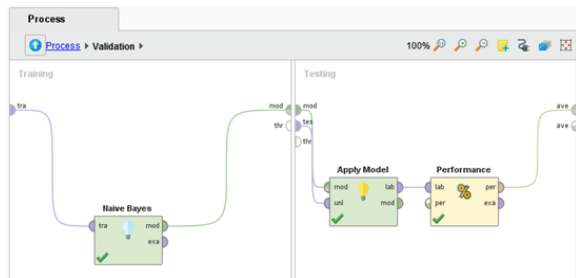
Gambar. 3. Implementasi Algoritma Naive Bayes
