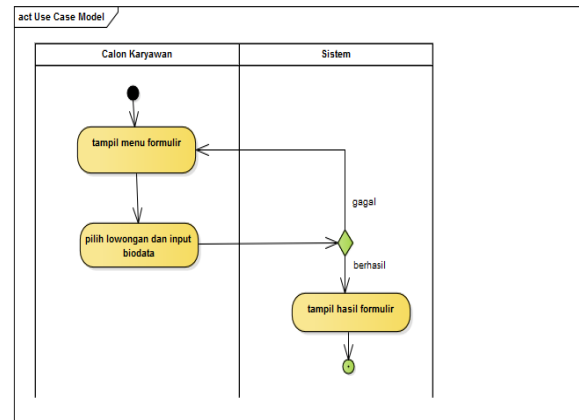
Gambar 3. Activity diagram isi formulir
