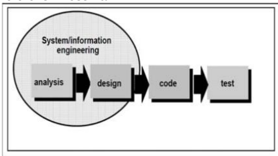
Gambar 1. Fase Waterfall
