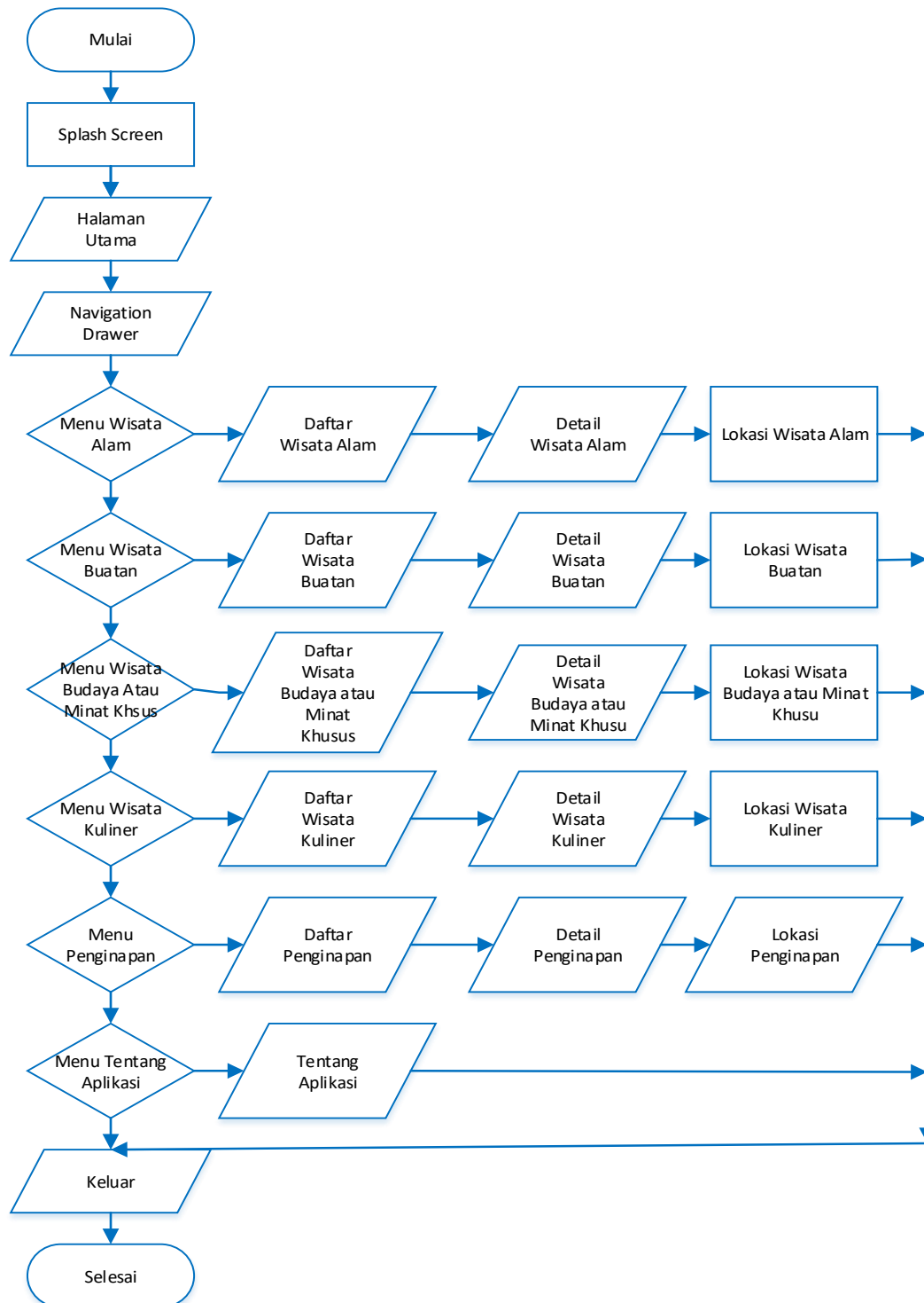
Gambar 9. Flowchart White Box Testing
