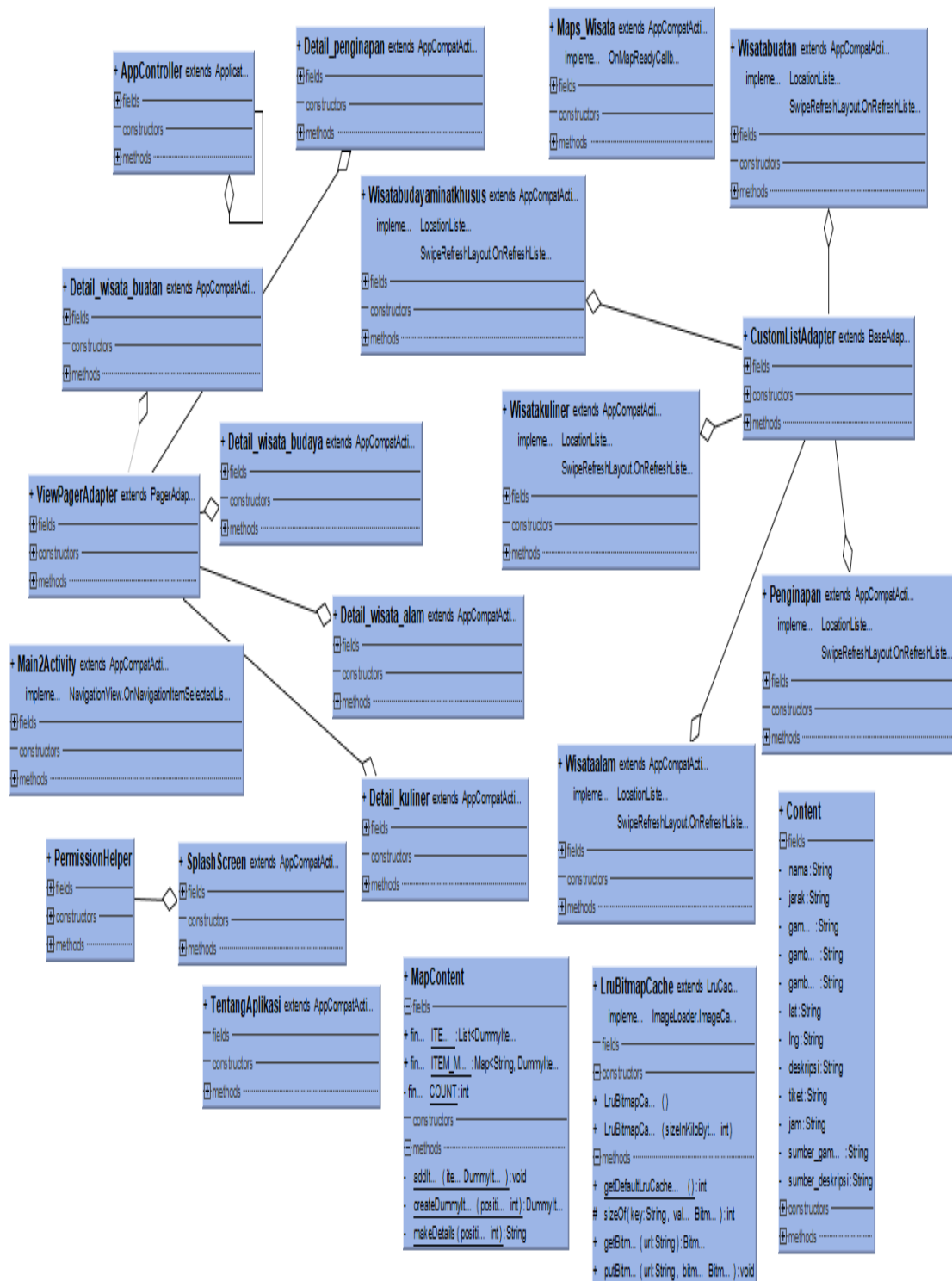
Gambar 8. Class Diagram
