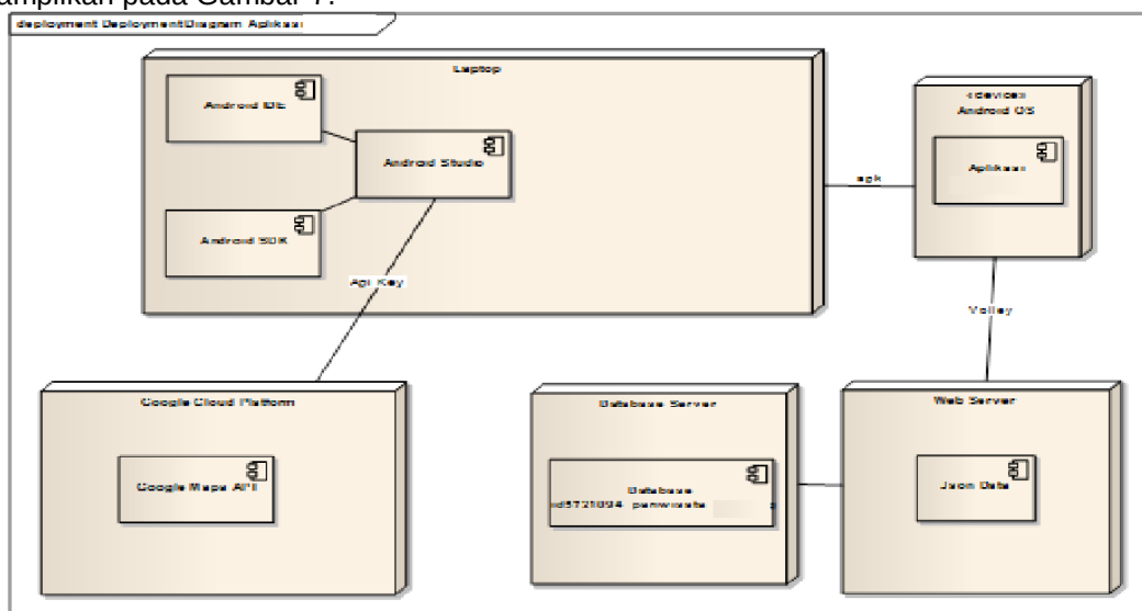
Gambar 7. Deployment Diagram
