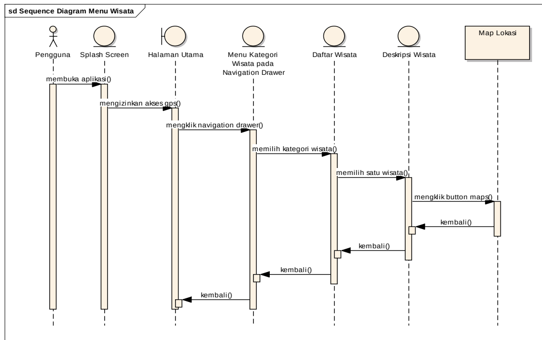
Gambar 6. Sequence Diagram
