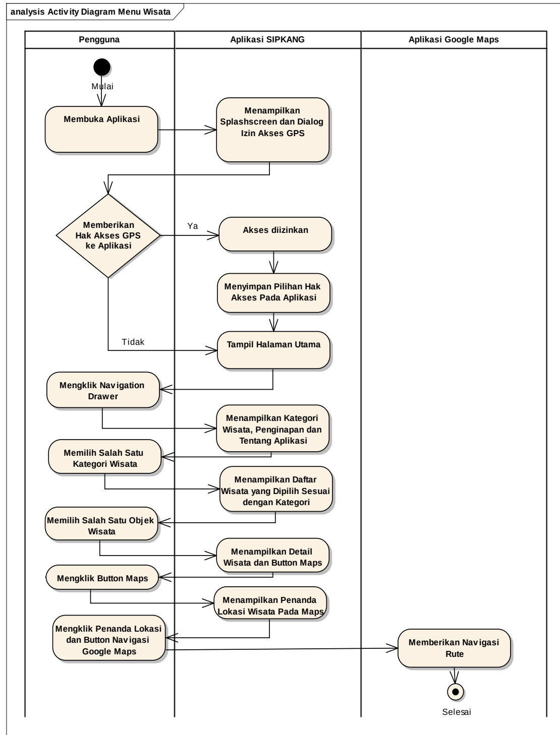
Gambar 5. Activity Diagram
