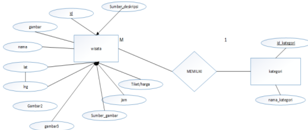
Gambar 3. ERD (Entity Relationship Diagram)
