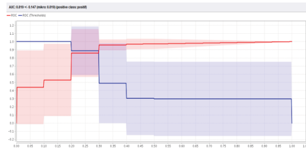
Fig. 3. Graph Area Under Curve (AUC) Naïve Bayes Algorithm after addition selection feature of Genetic Algorithm
