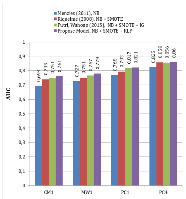
Figure 1. Chart of Comparison AUC values between Previous Model
