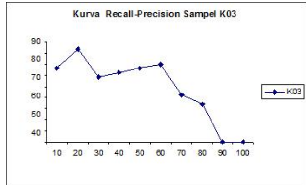
Gbr. 7 Kurva Recall-Precision Sampel K03
