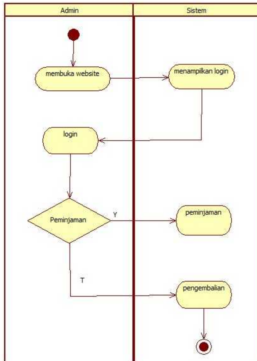
Gambar 4.6 Activity Diagram login admin
