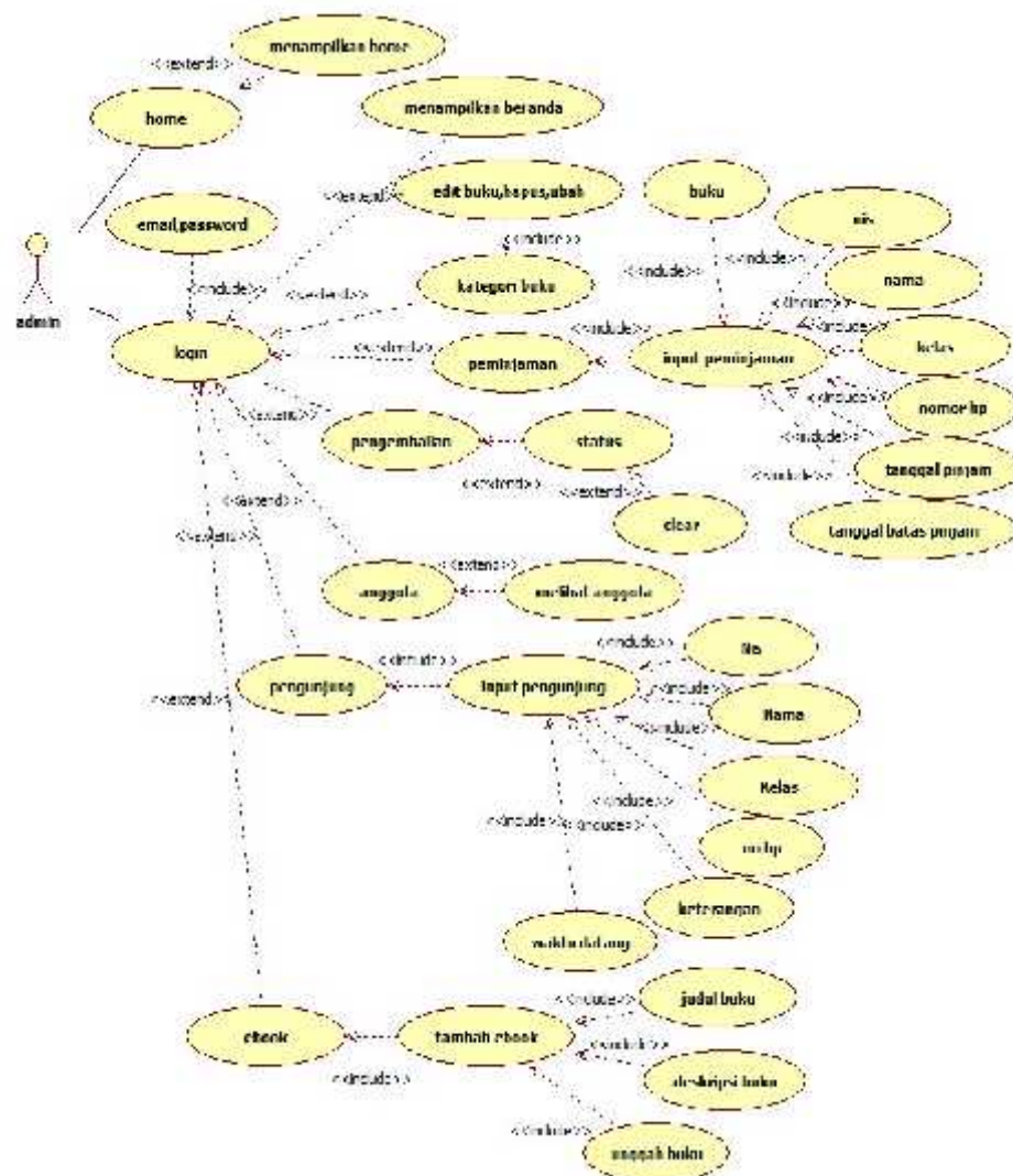
Gambar 4.2 Use Case Diagram Halaman Admin
