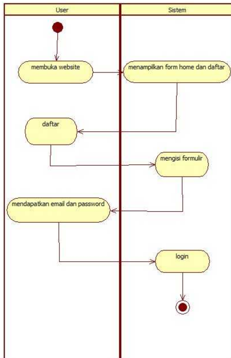
Gambar 4.3 Activity Diagram pendaftaran User
