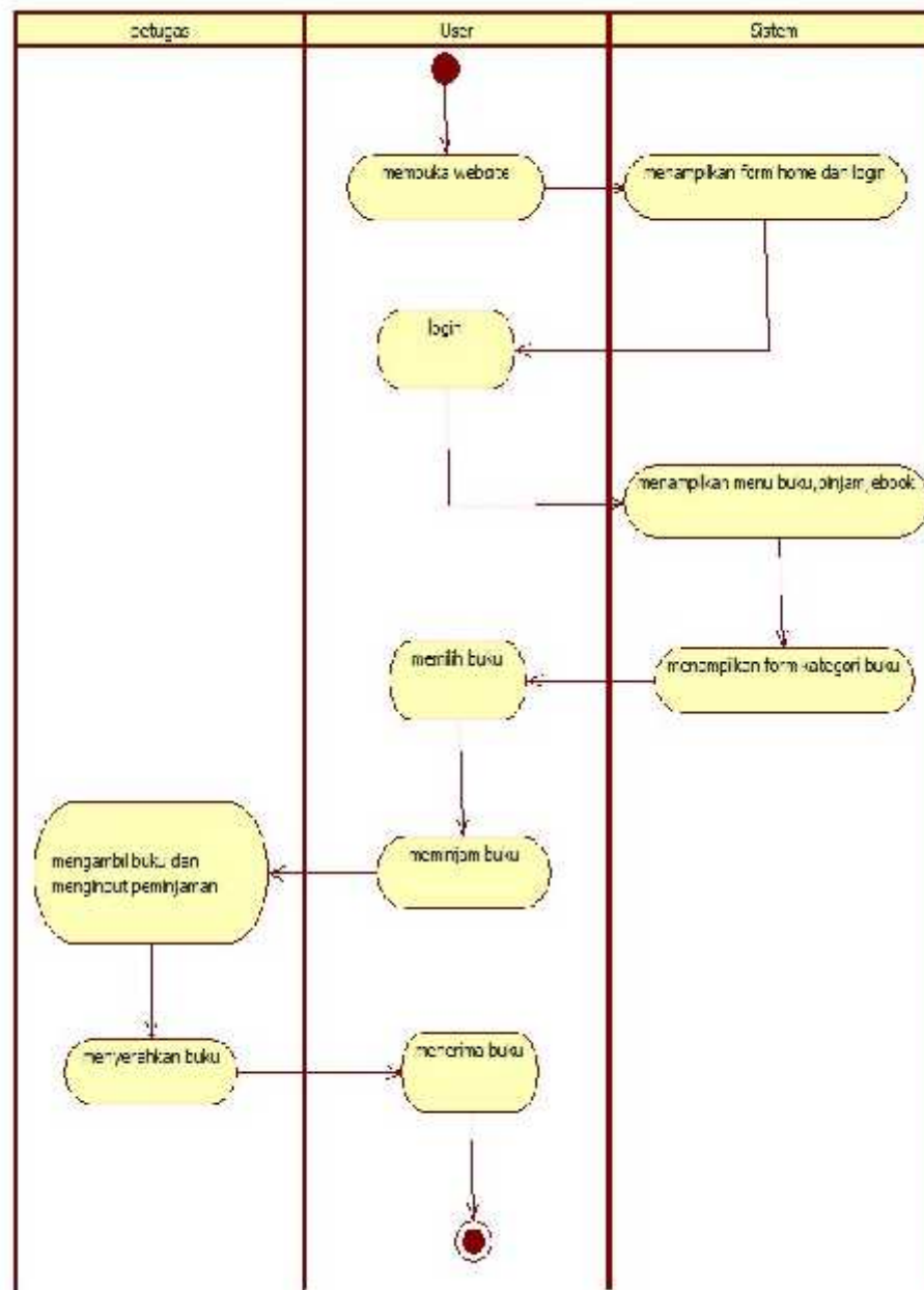
Gambar 4.4 Activity Diagram peminjaman User
