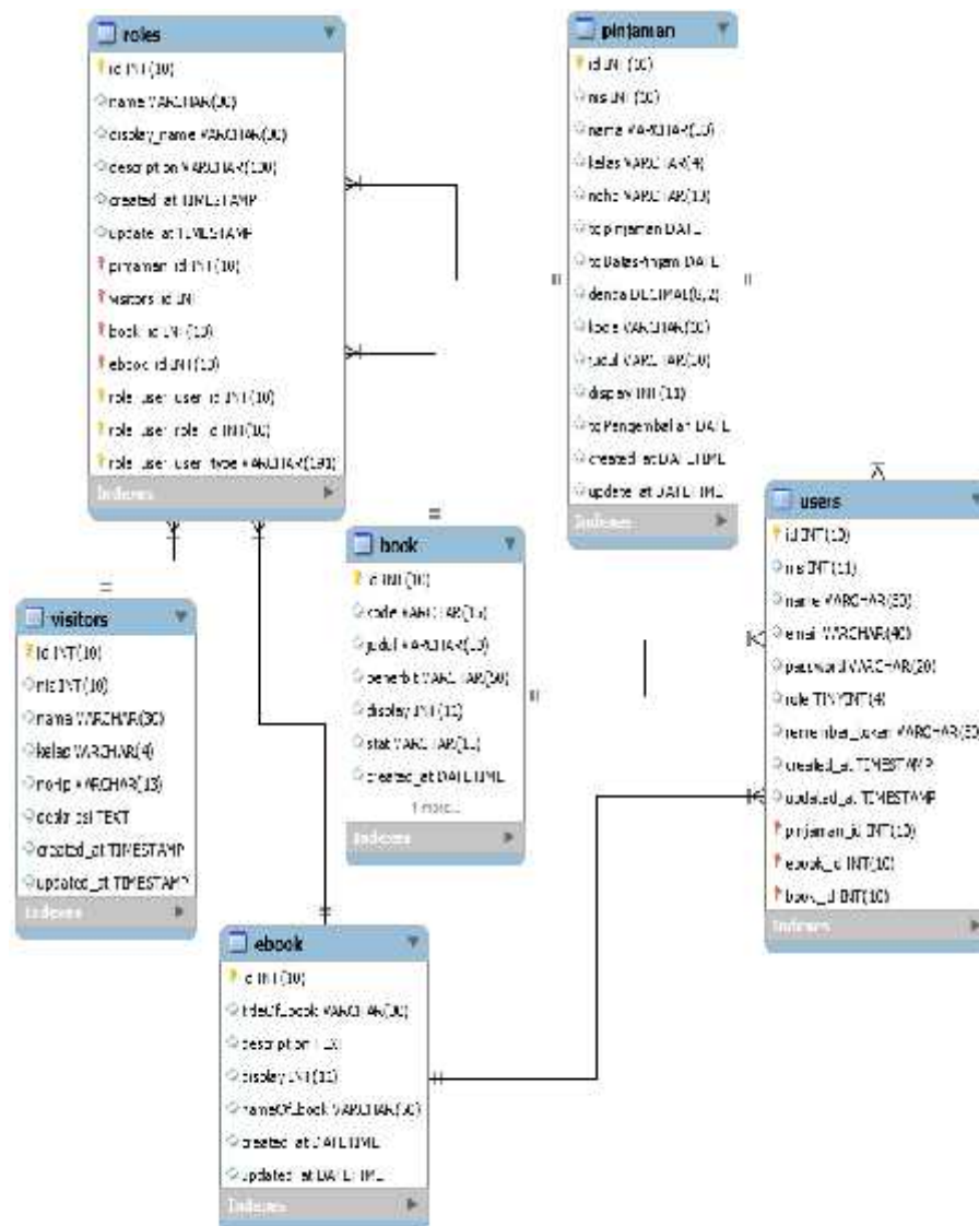
Gambar 4.8 Logical Record Structure
