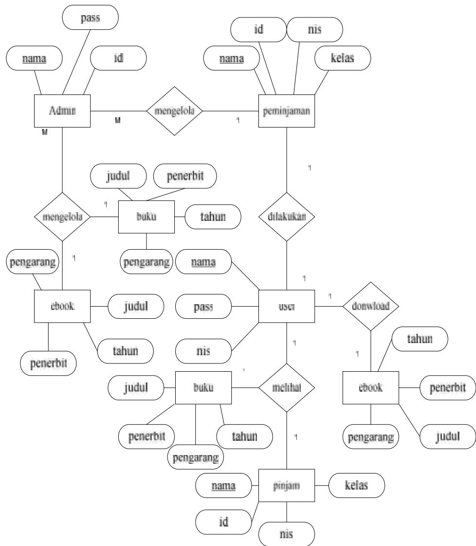
Gambar 4.7 Entity Relationship Diagram
