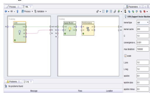
Gambar 7. Model Pengujian validasi Support Vector Machine
