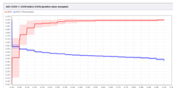
Gambar 10. Kurva ROC dengan Metode Support Vector Machine berbasis Particle Swarm Optimization (PSO)
