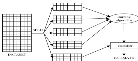
Gambar 2. K-Fold Cross-validation
