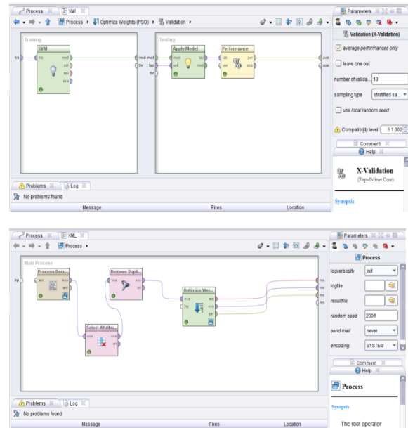
Gambar 9. Model Pengujian validasi Support Vector Machine berbasis Particle Swarm Optimization (PSO)
