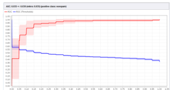
Gambar 11. Kurva ROC dengan Support Vector Machine dan Support Vector Machine berbasis Particle Swarm Optimization
