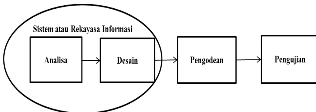
Gambar 1. Model waterfall
