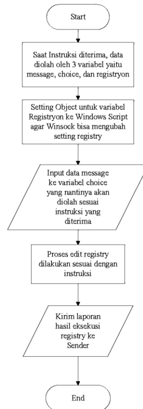
Gambar 11 Proses Saat Receiver Menerima Instruksi
