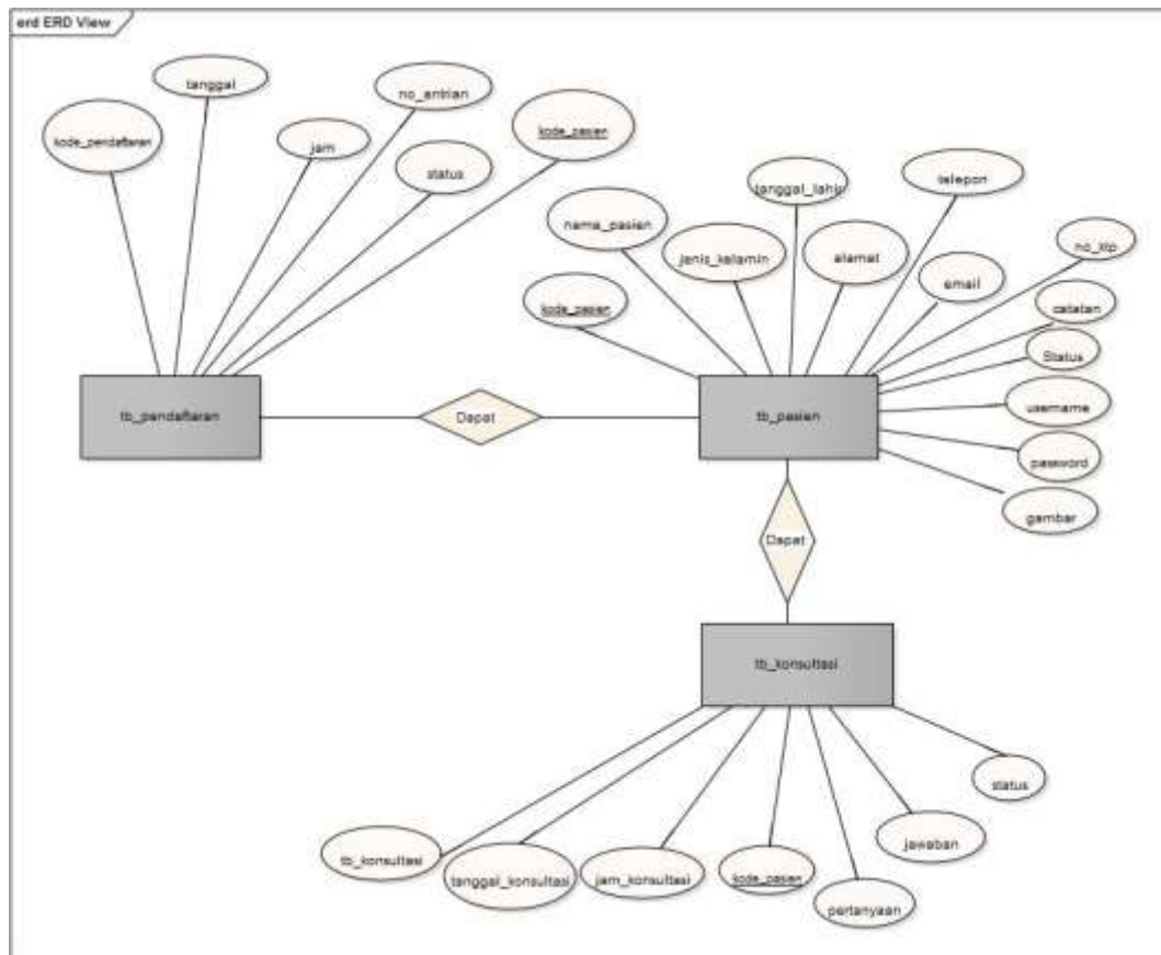
Gambar IV.1 Entity Relationship Diagram
