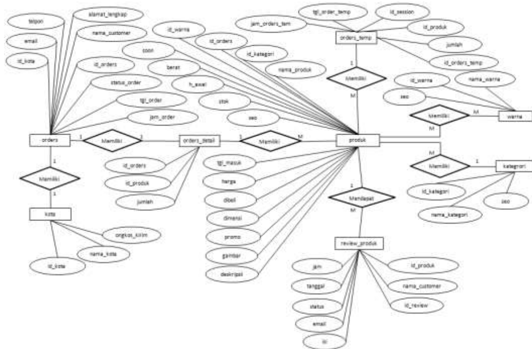
Gambar IV.17 Entity-relation Diagram
