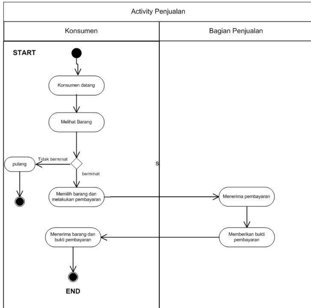
Gambar III.3. Activity Diagram Penjualan Sistem Berjalan
