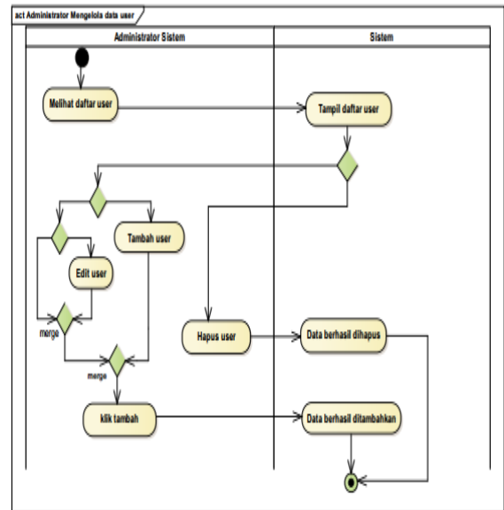
Gambar 5. Activity Diagram Mengelola Data user
