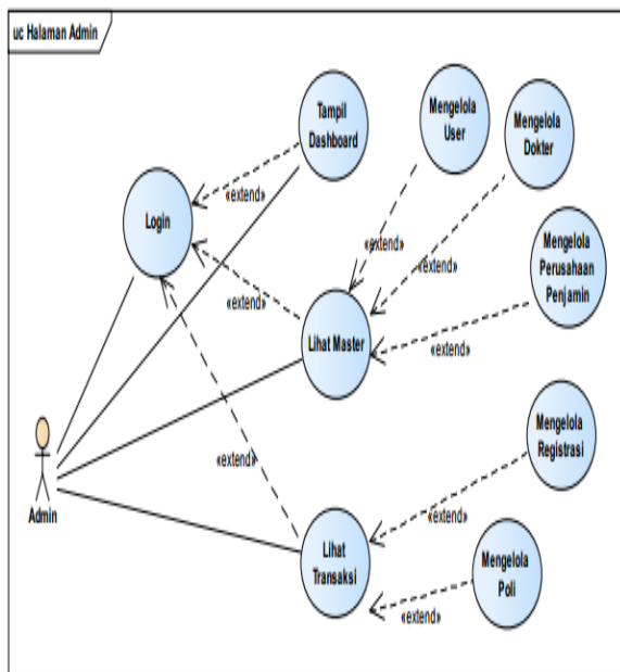
Gambar 4. Use Case Diagram Halaman Administrator System
