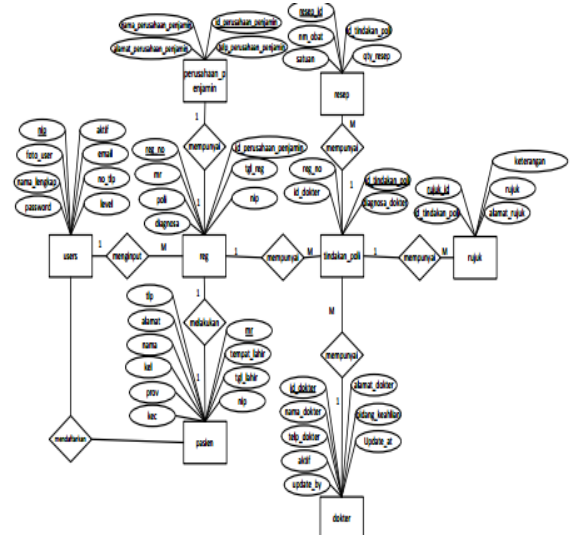
Gambar 14. Entity Relationship Diagram
