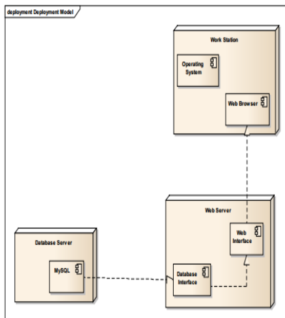
Gambar 8. Deployment Diagram
