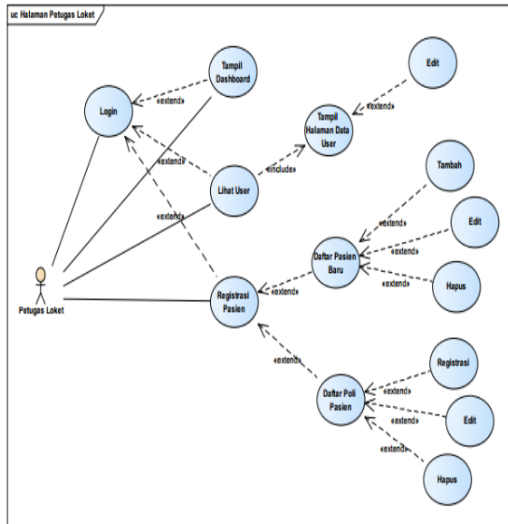
Gambar 3. Use Case Diagram Halaman Petugas Loket
