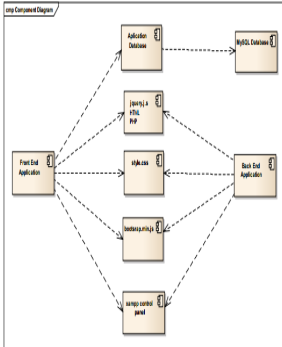
Gambar 7. Component Diagram
