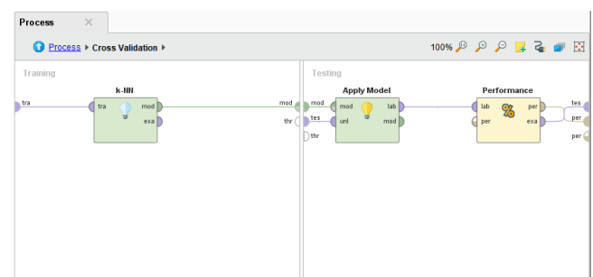
Gambar 5. Model Validasi KNN
