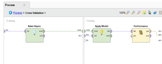
Gambar 3. Model Validasi Naive Bayes
