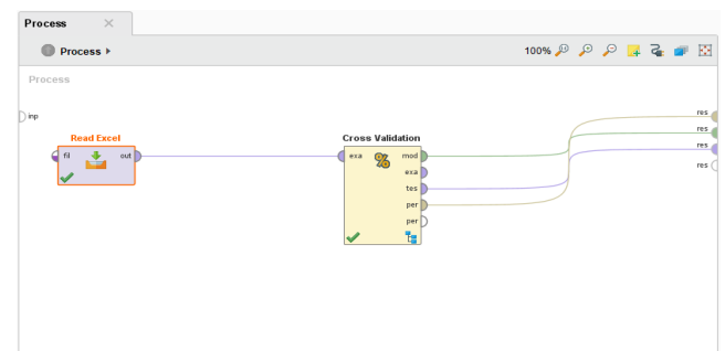
Gambar 4. Model Prose KNN
