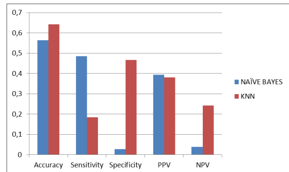
Gambar 6. Perbedaan Nilai Accuracy, Sensitivity, Specificity, PPV, dan NPV Algoritma Naïve Bayes dan KNN
