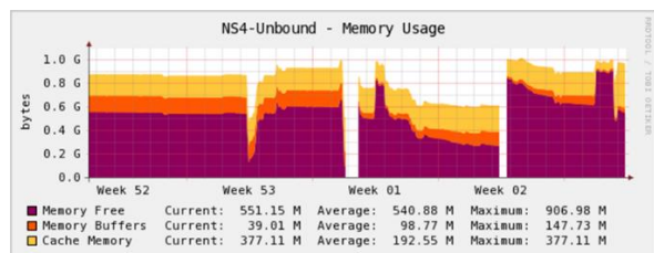
Gambar 24. Utilisasi memori (RAM server Unbound
